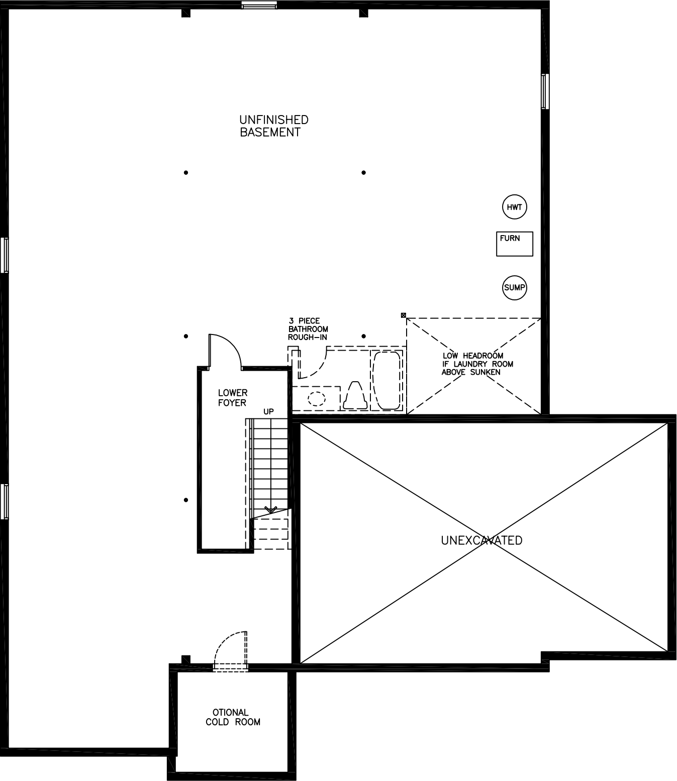
BASEMENT PLAN
