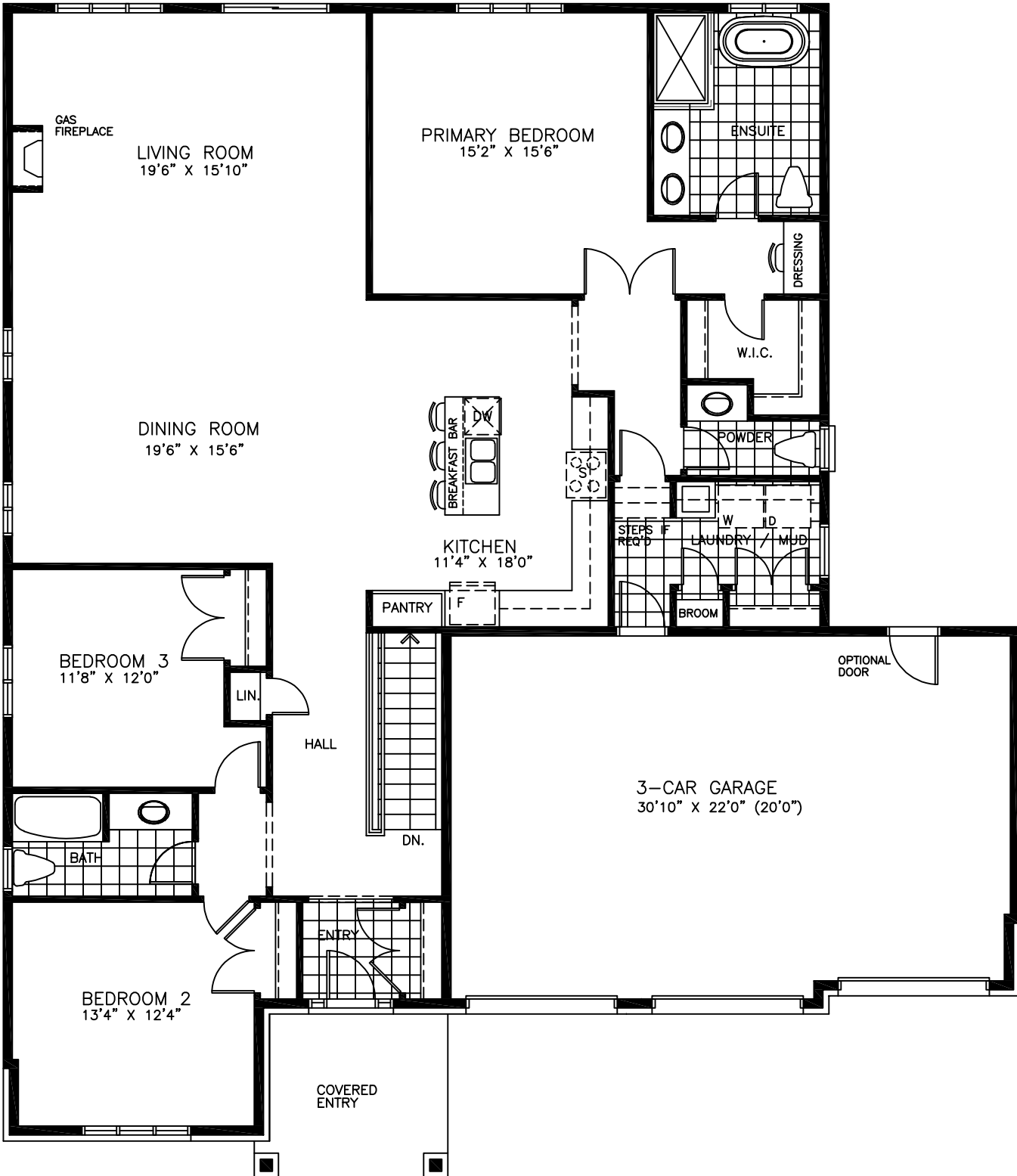
GROUND FLOOR PLAN GFA = 2200 SF MODEL TYPE B-2200 JULY 5 2026
